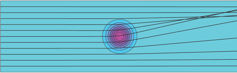
Figure 10. Bending of a beam of parallel rays by a strong Gaussian vortex \xi = \xi_0 \exp(-(r/\ell)^2) , with \xi_0/\sqrt{gk} = 5/\pi and \ell k = 40 . In this illustration the vortex is unrealistically strong in order to show the ray pattern; realistic vortices produce much smaller deflections.
