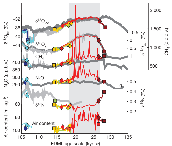
Figure 2 | Reconstructed records from the NEEEM ice core. The reconstructed records of \delta^{18}\text{O}_{\text{ice}} , \delta^{18}\text{O}_{\text{atm}} (reversed scale) \text{CH}_4 , \text{N}_2\text{O} , \delta^{15}\text{N} and air content (reversed scale) on the EDML1 timescale 12 . Zone 1 (cyan) is seen to contain a fold while zone 2 (green) and zone 3 (orange) are reversed and cover identical time periods. NGRIP records (light grey) and EDML records (dark grey) are included where they are available. The \text{CH}_4 , \text{N}_2\text{O} and air content records contain spikes from 127 to 118.3 kyr BP (shaded grey).
